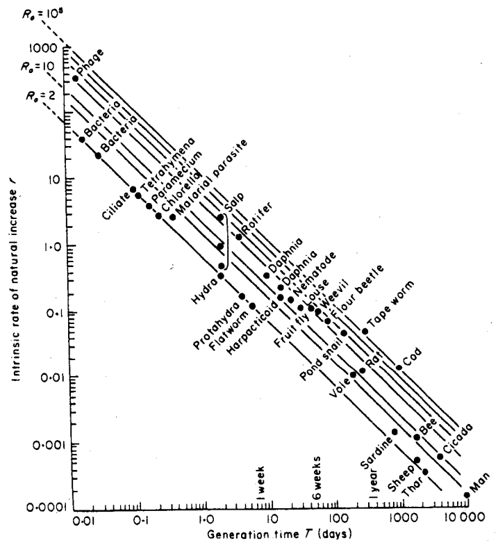
Fig. 3.2. The relationship of the intrinsic rate of natural increase and generation time, with diagonal lines representing values of R_0 from 2 to 10^5 , for a variety of organisms (from Heron, 1972).
